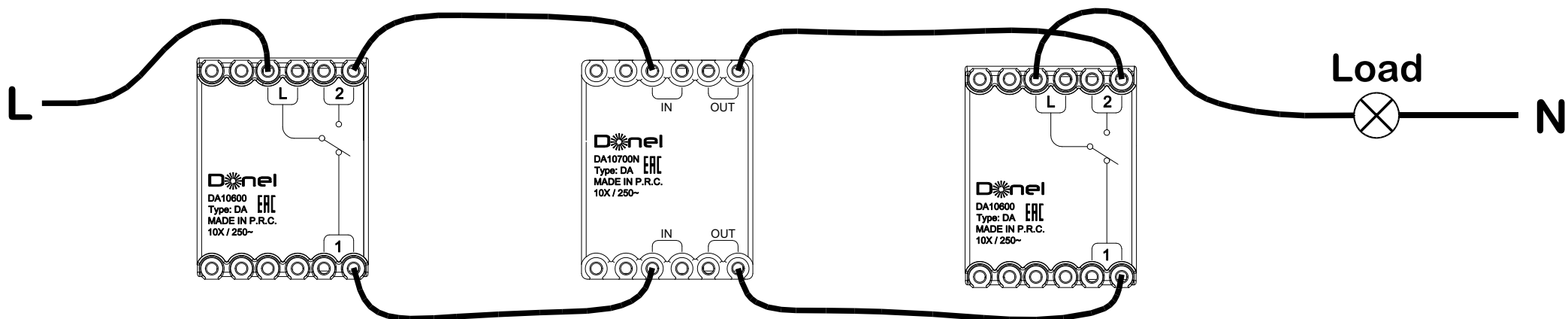
1 Gang 2 Way Switch
